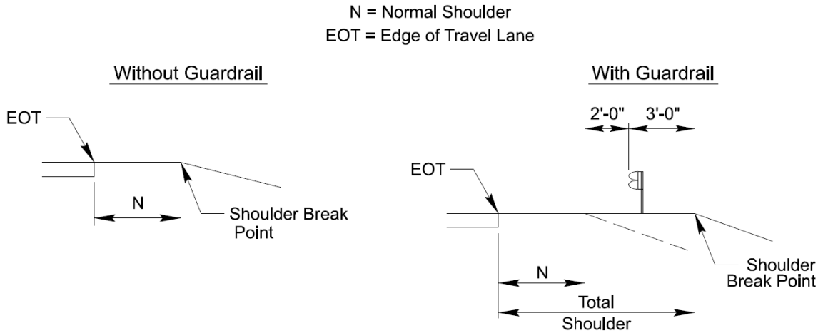
Figure 4-2 Normal and Total Shoulder Width for Arterials, Interstates, and Freeways
