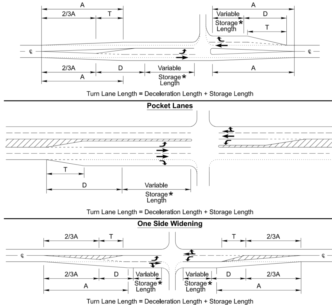
Figure 8-11 Recommended Treatment for Turn Lanes Symmetrical Widening
